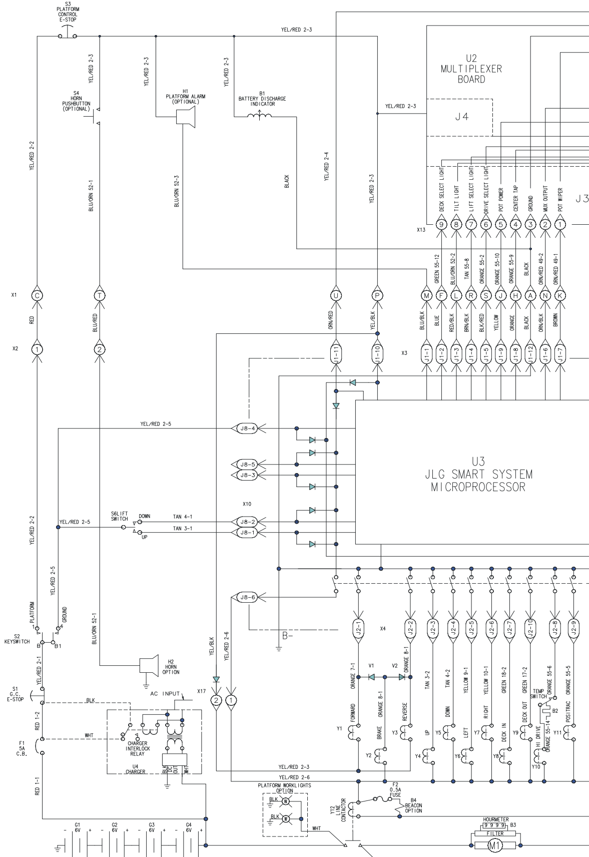
FIGURE 7-2.ELECTRICAL SCHEMATIC (PROPORTIONAL CONTROL MACHINES)
