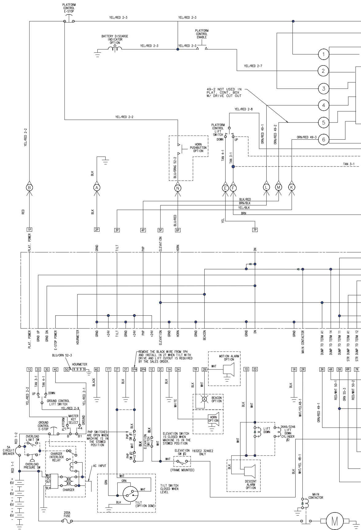
FIGURE 7-1.ELECTRICAL SCHEMATIC (STANDARD CONTROL MACHINES)
