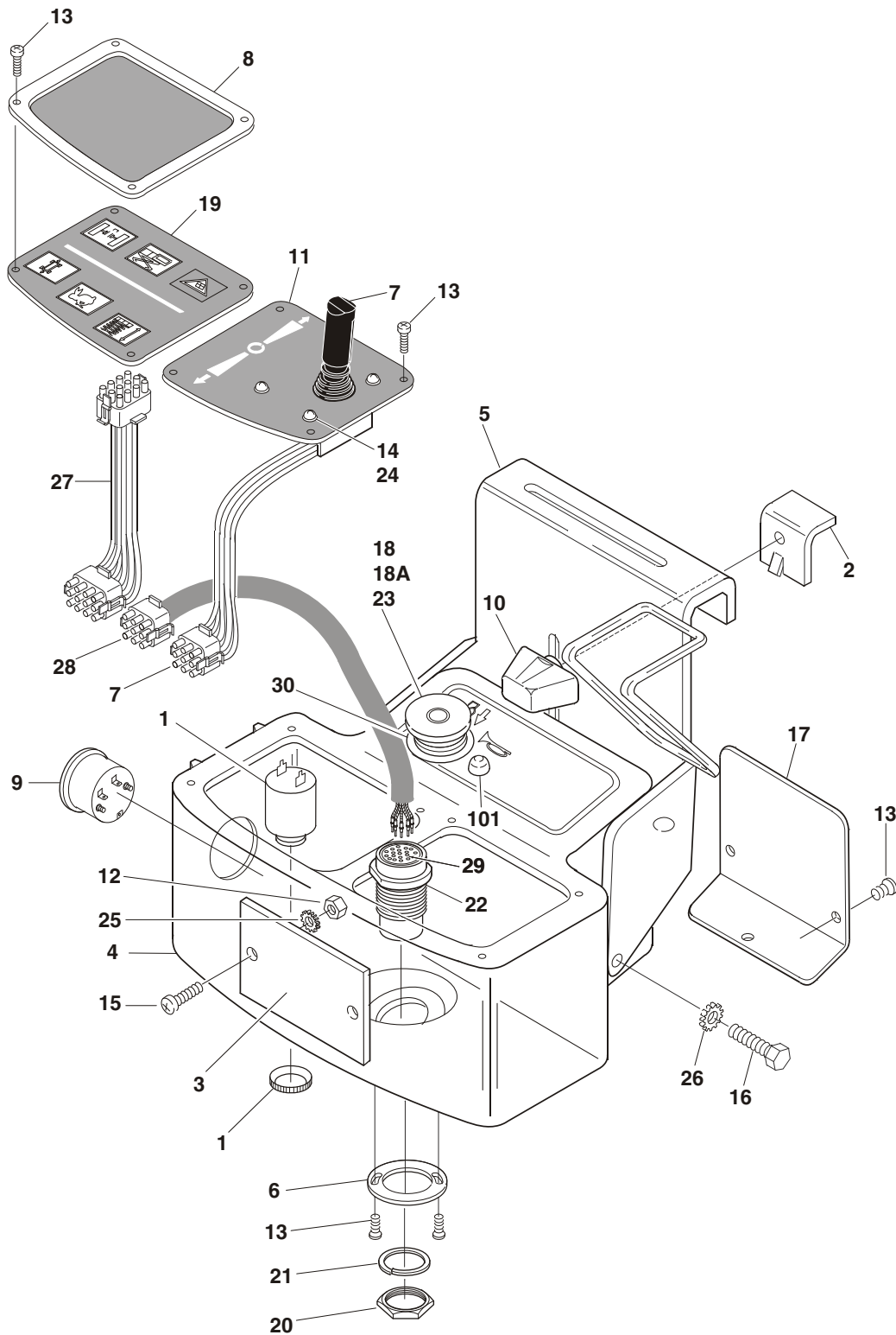
FIGURE 4-9.PLATFORM CONSOLE BOX ASSEMBLIES (PROPORTIONAL CONTROL MACHINES)
