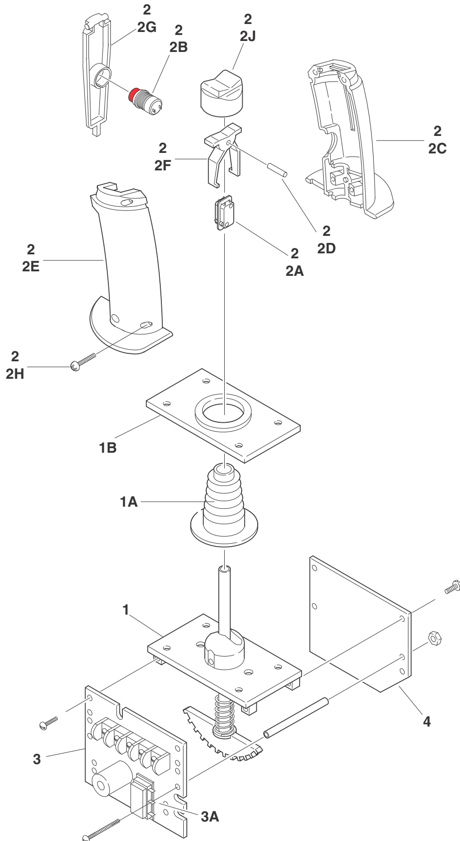
FIGURE 4-10. CONTROLLER ASSEMBLY (STANDARD CONTROLS MACHINES)
