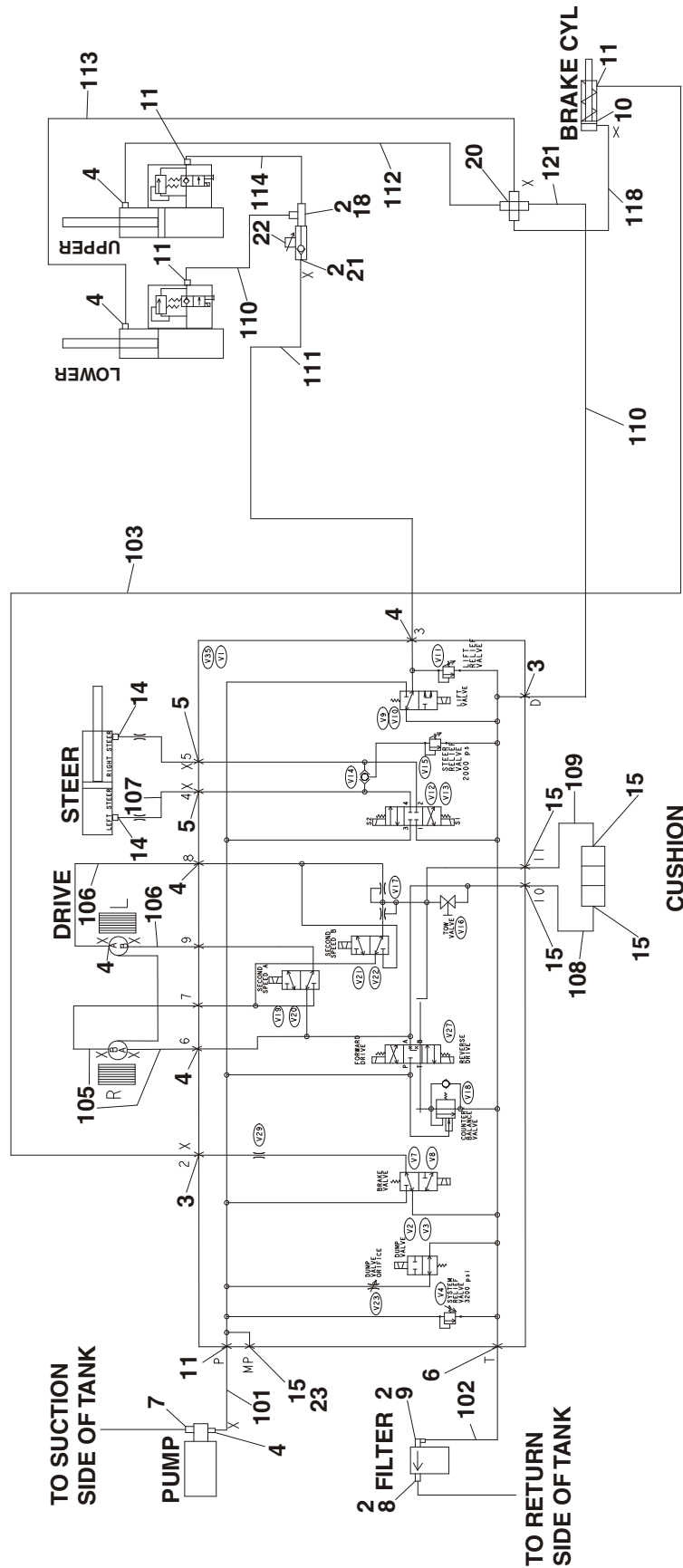
FIGURE 6-5.HYDRAULIC DIAGRAM - 2632E2 WITH STANDARD CONTROLS
