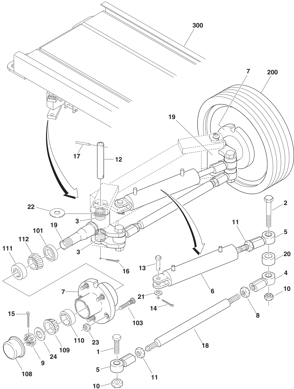
FIGURE 1-4. FRAME AND STEERING INSTALLATIONS - 2032E2/2632E2/2646E2/3246E2
