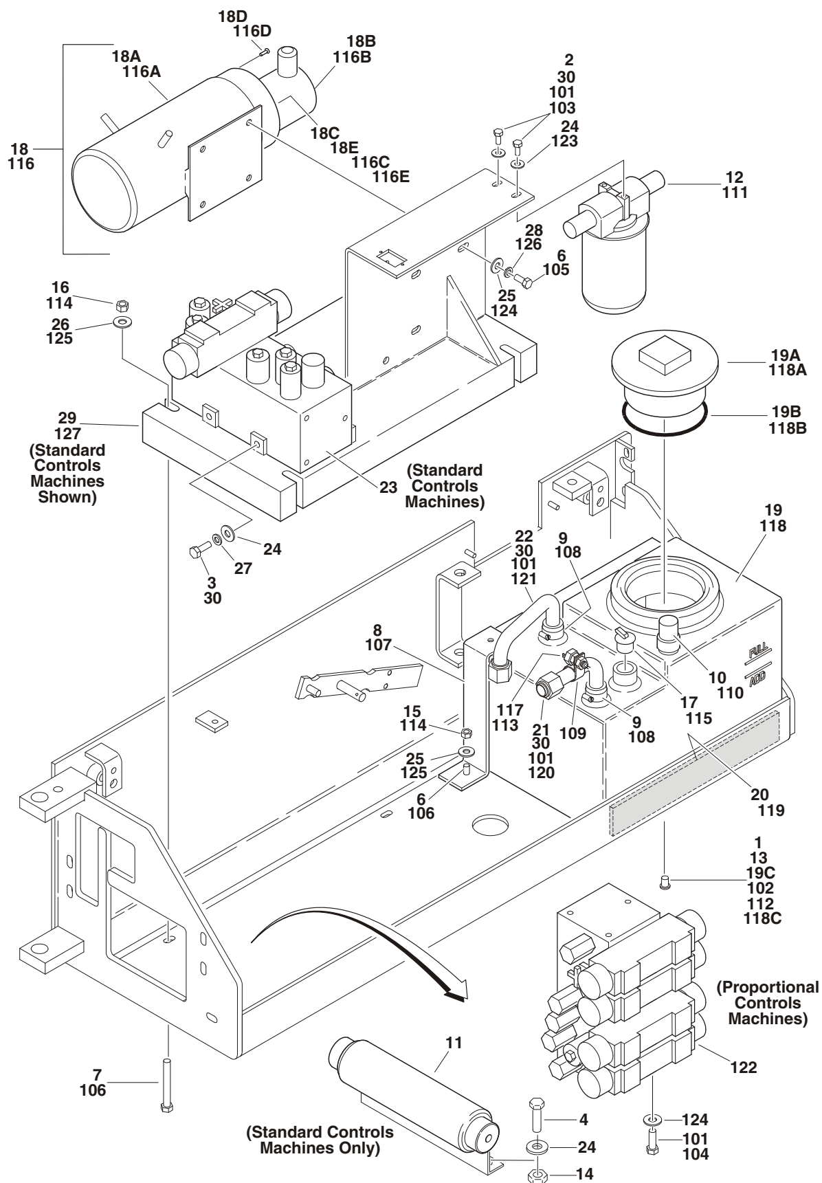
FIGURE 2-2. HYDRAULIC COMPONENT INSTALLATIONS - 2032E2/2632E2/2646E2/3246E2
