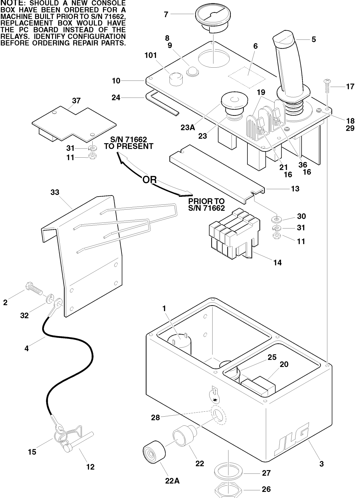
FIGURE 4-8.PLATFORM CONSOLE BOX ASSEMBLIES (STANDARD CONTROL MACHINES)
