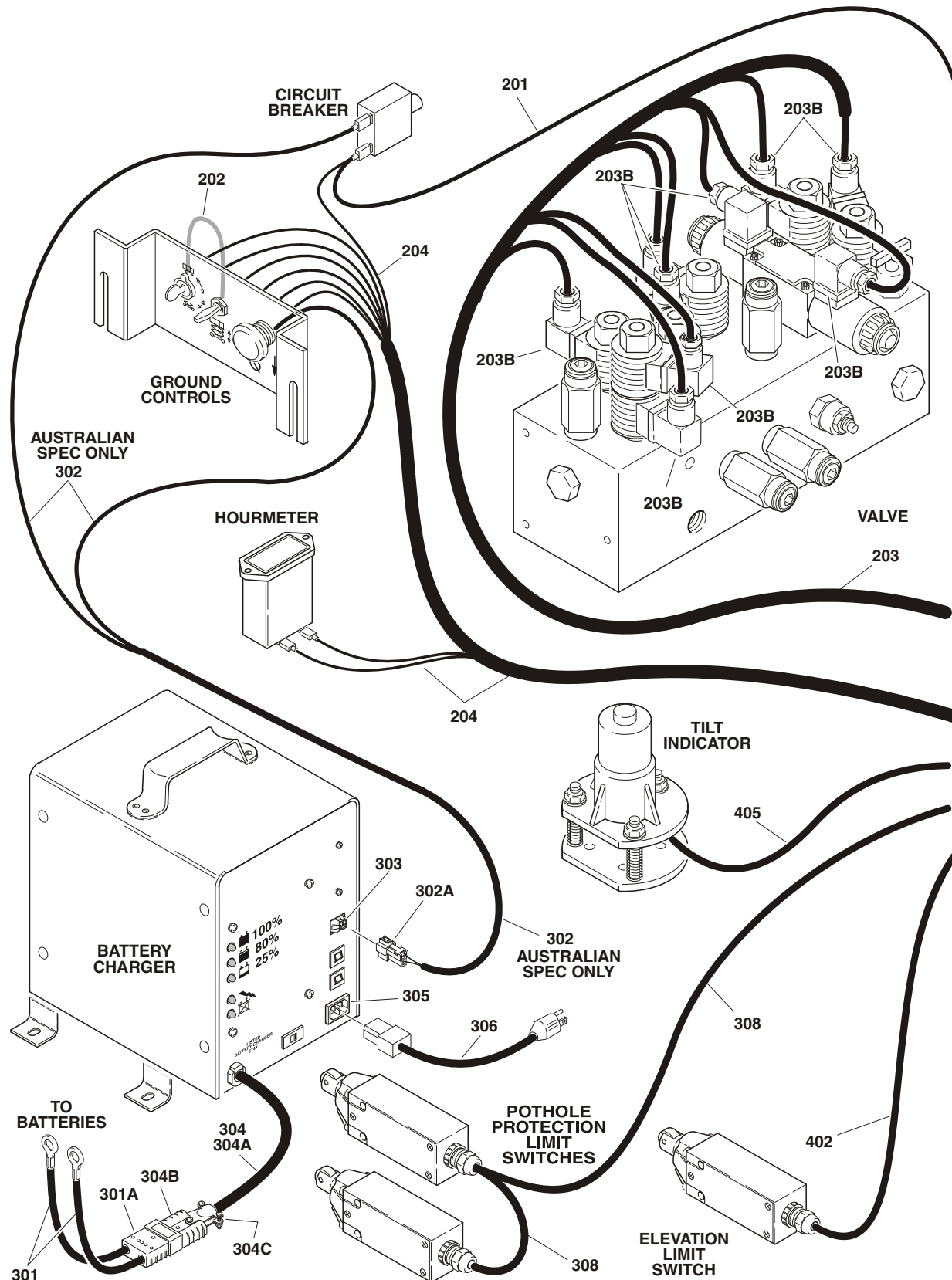
FIGURE 7-3. ELECTRICAL COMPONENTS INSTALLATION (STANDARD CONTROL MACHINES)
