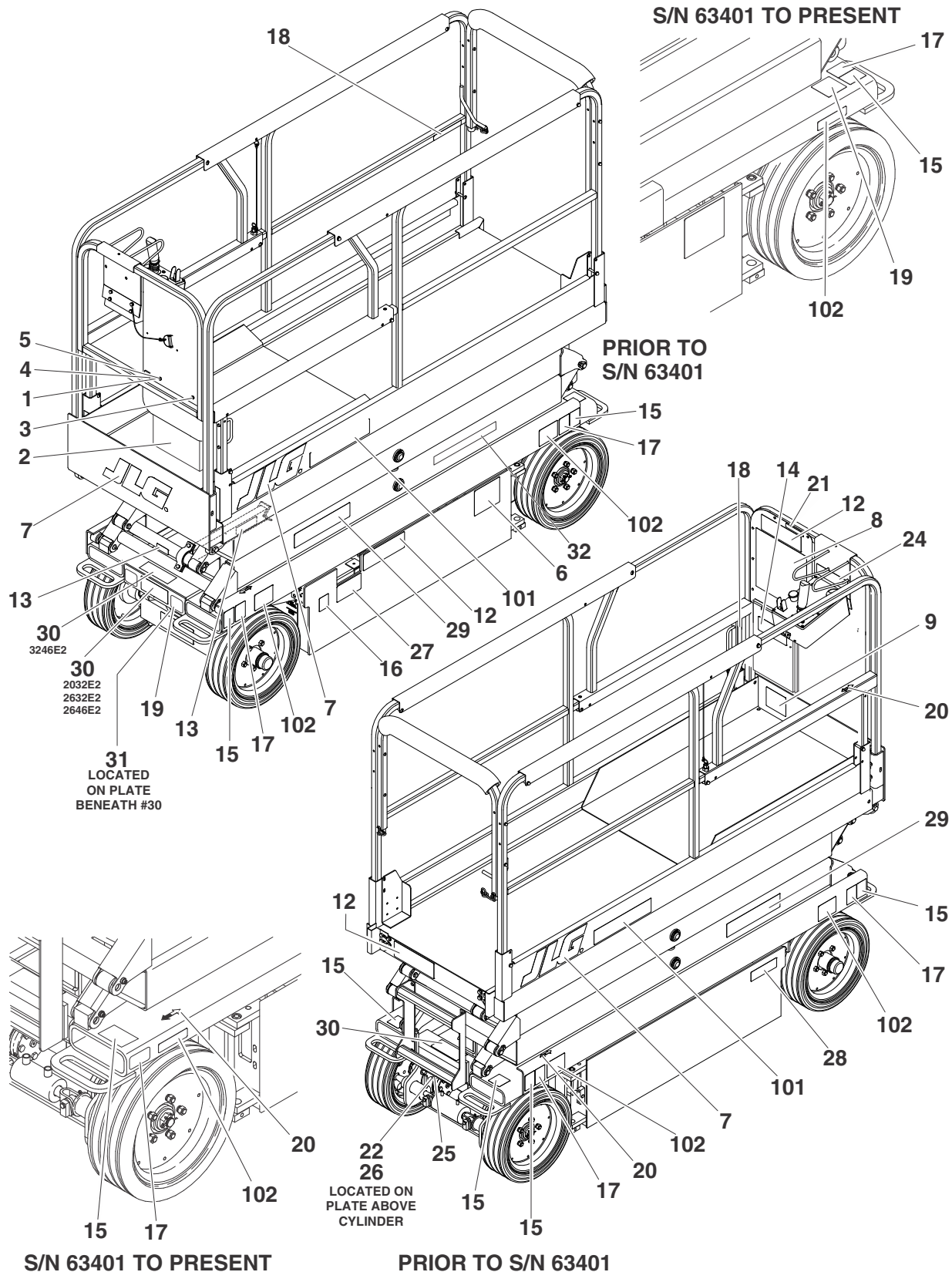
FIGURE 8-4.DECALS INSTALLATION - 2032E2&2632E2&2646E2&3246E2 (COUNTRY SPEC)
