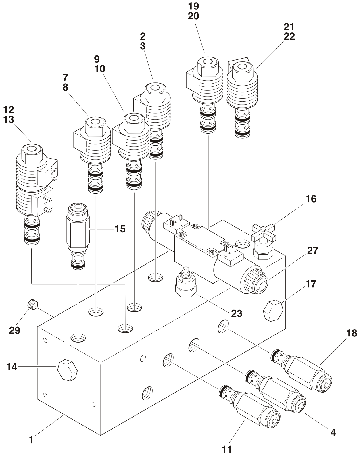
FIGURE 2-3. VALVE ASSEMBLY - STANDARD CONTROLS MACHINES
