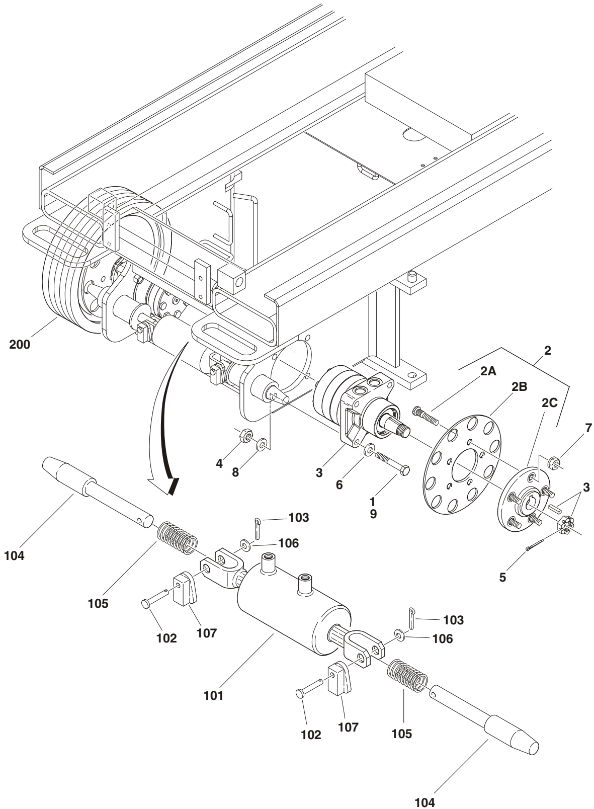
FIGURE 1-5. WHEEL DRIVE AND BRAKE INSTALLATIONS - 2032E2/2632E2/ 2646E2/3246E2
