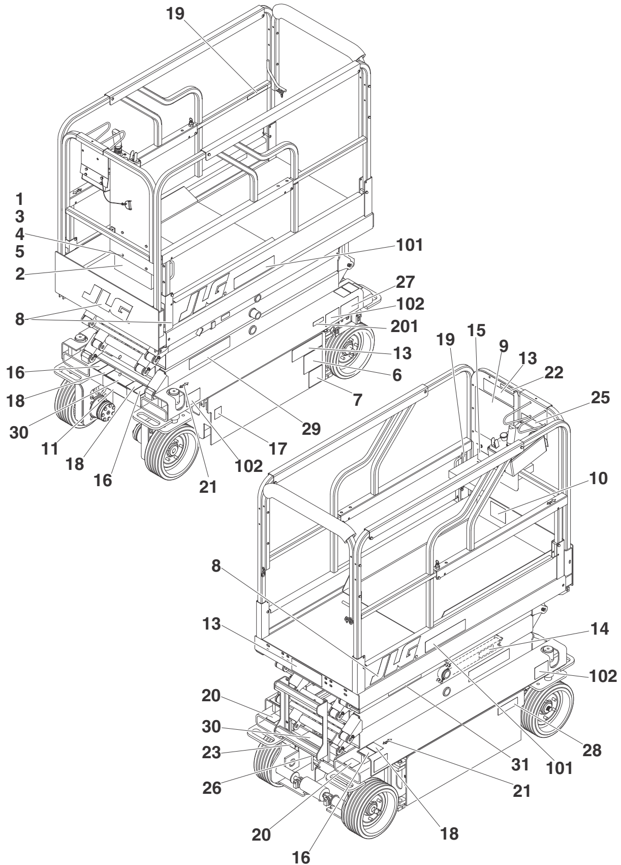
FIGURE 8-1.DECALS INSTALLATION - 1532E2 & 1932E2 (COMMON)
